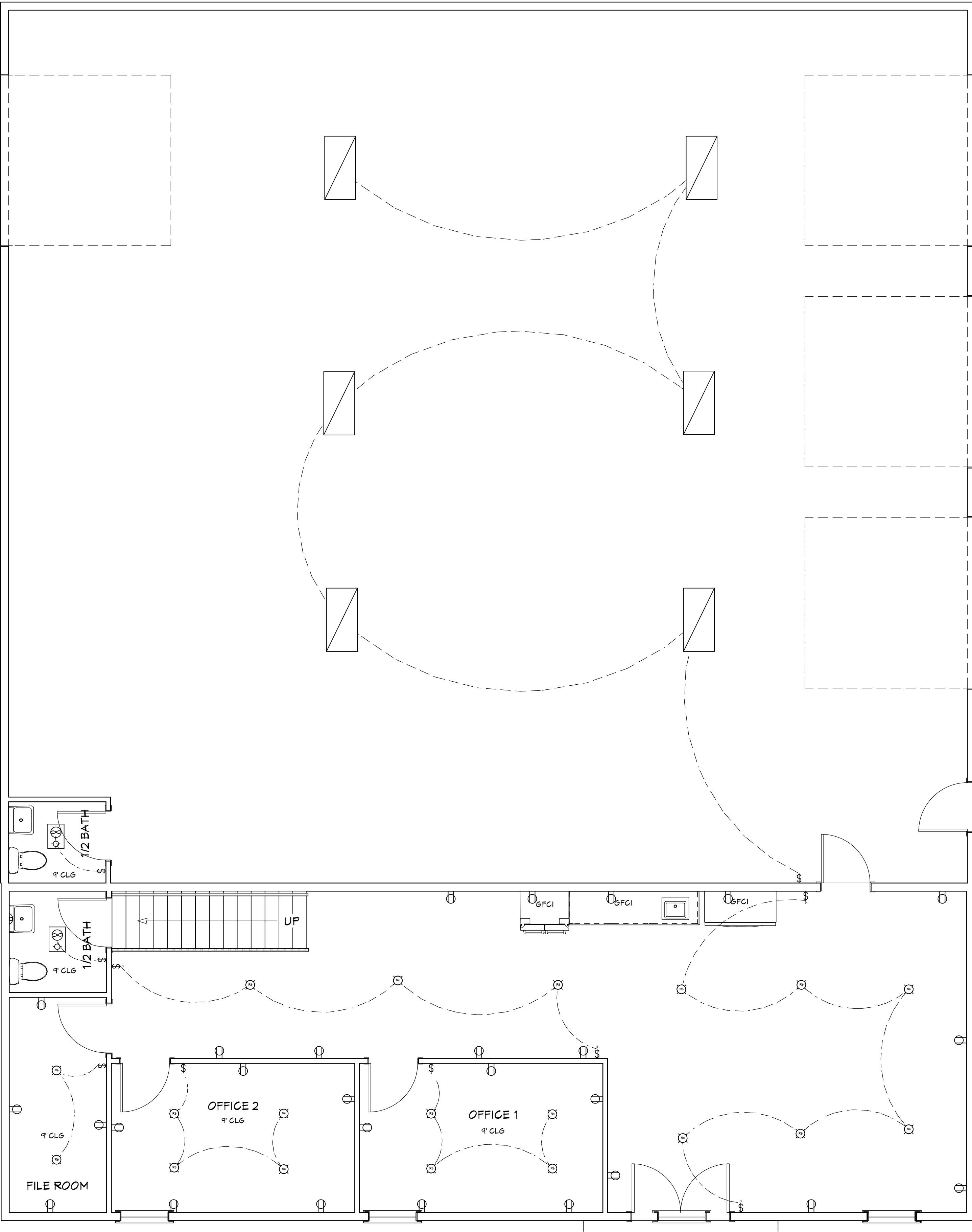
ELECTRICAL PLAN VIEW 1/4 IN = 1 FT
