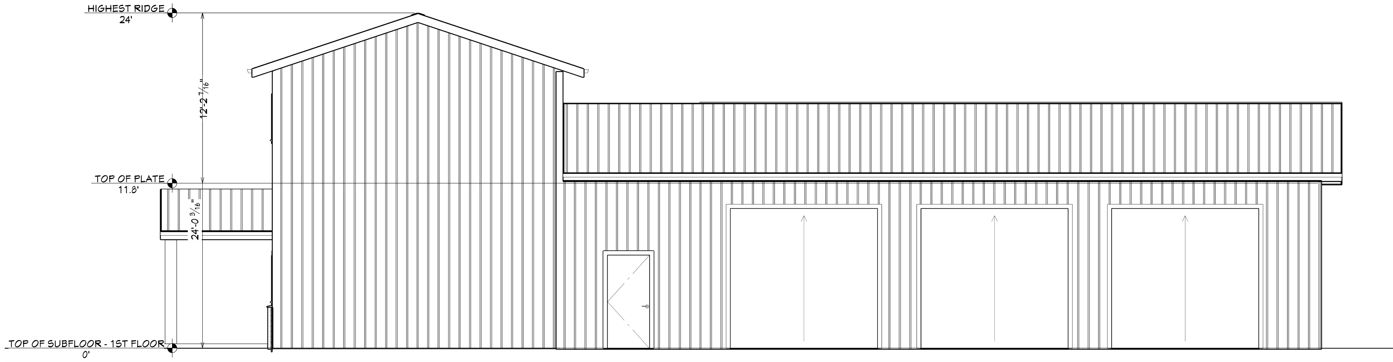
E4 EXTERIOR ELEVATION RIGHT 1/4 IN = 1 FT
