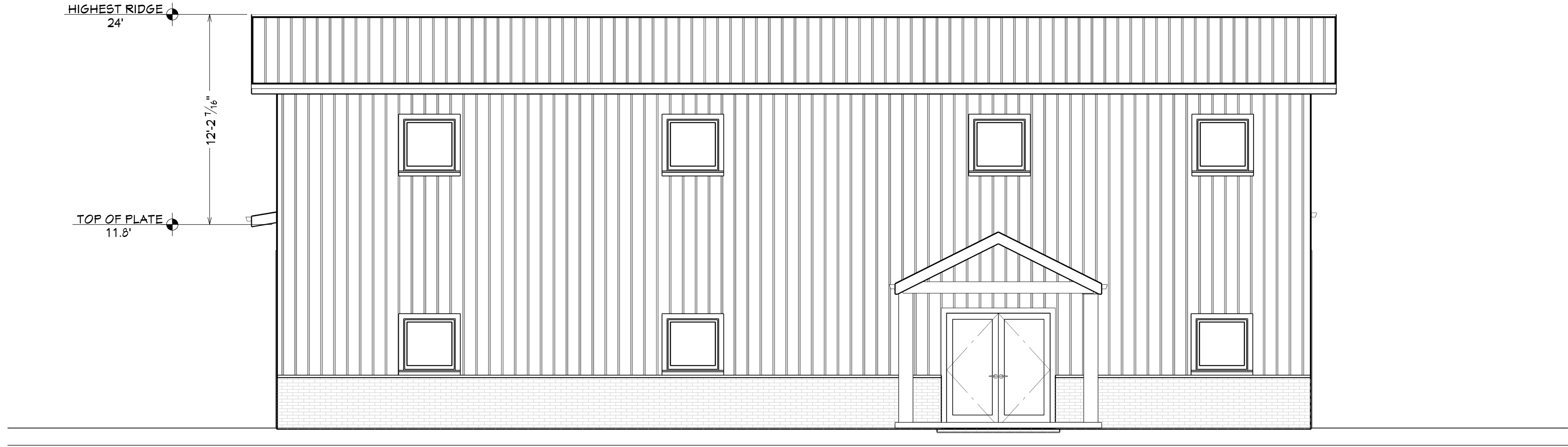
E1 EXTERIOR ELEVATION FRONT 1/4 IN = 1 FT
