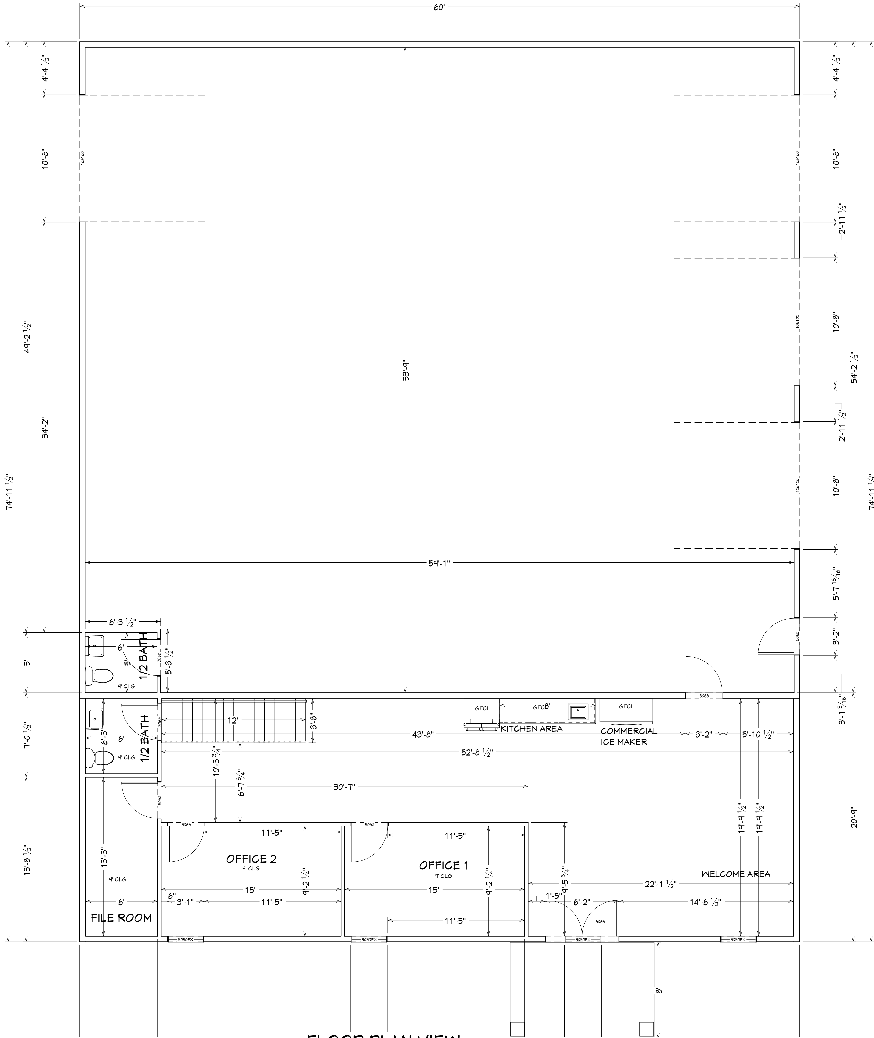
FLOOR PLAN VIEW 1/4 IN = 1 FT
