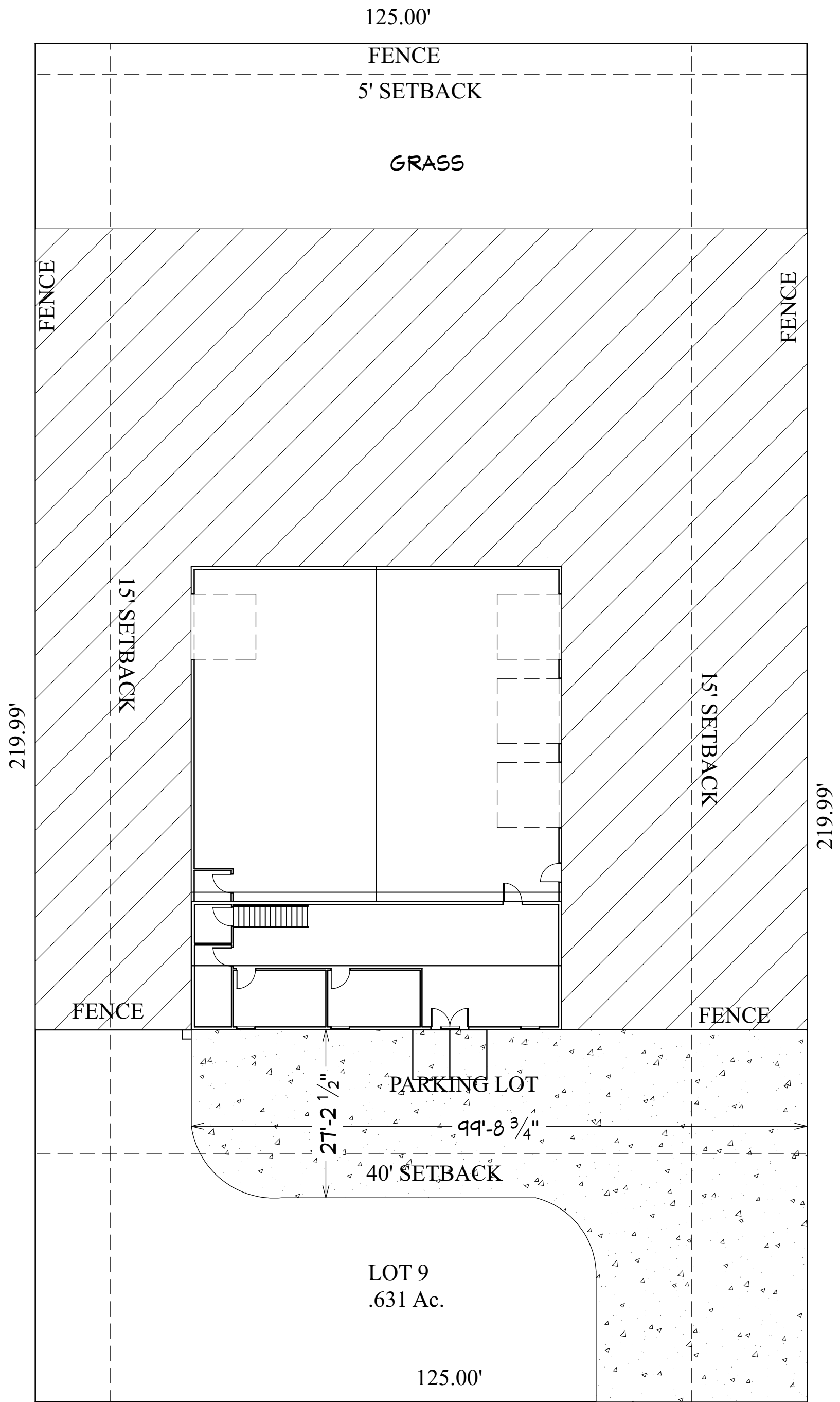
SITE PLAN 1/16 IN = 1 FT
